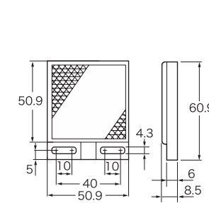
Standard reflector V-61 (Standard, LED type)
